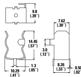
106 001 Device Dimensions
